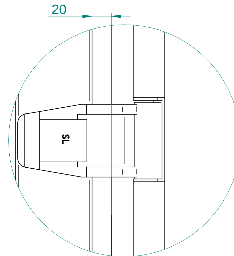
DETAIL A 1:2
